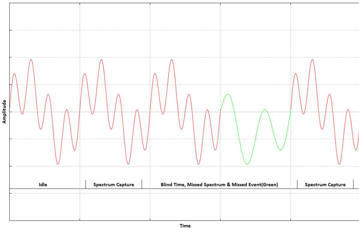
In this image, we see an event missed due to the blind time between spectrum sampling. With Real-Time spectrum analysis we can prevent this and capture ALL events.
